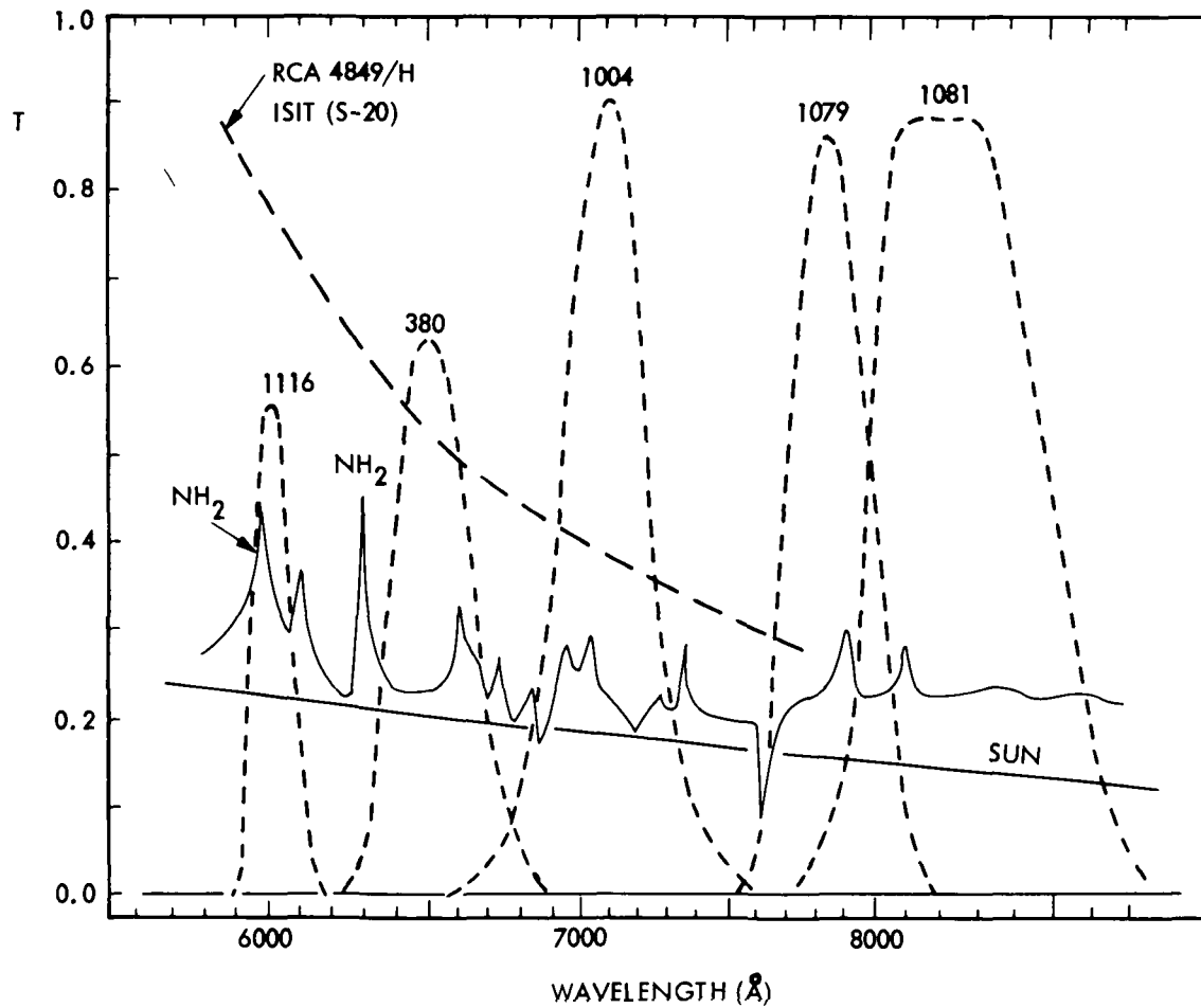
Figure 3b. As Figure 3a but for the red part of the spectrum.
